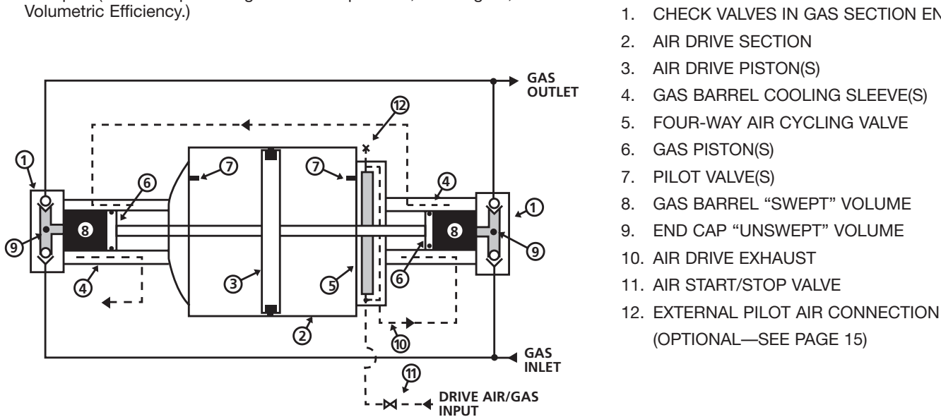
Figure 1. Typical Double Acting, Single Drive, Single Stage Unit (Model 5G-DS-Ratio)
